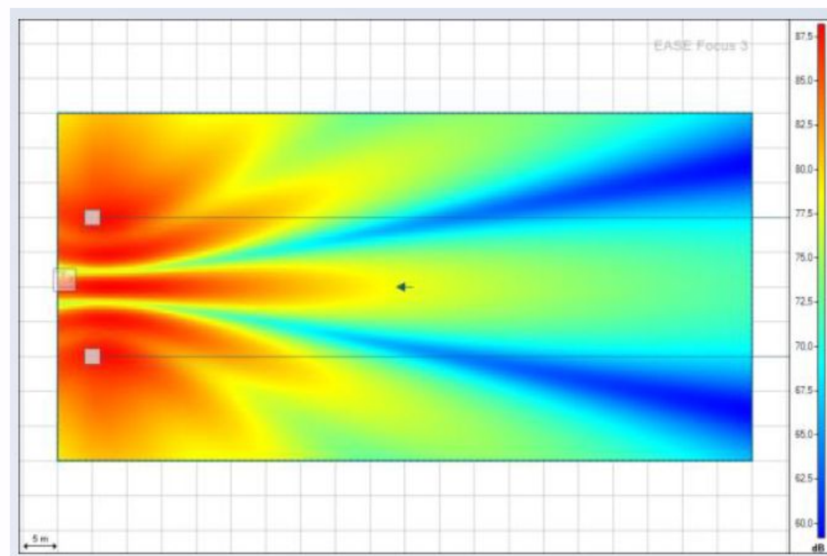
Simulation Subwoofer
